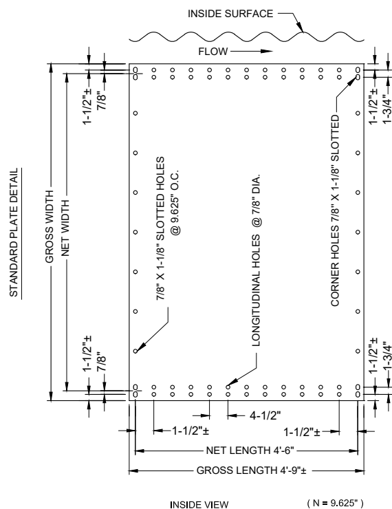
FIGURE 2. PLATE MARKINGS &amp; DETAILS DRAWING
