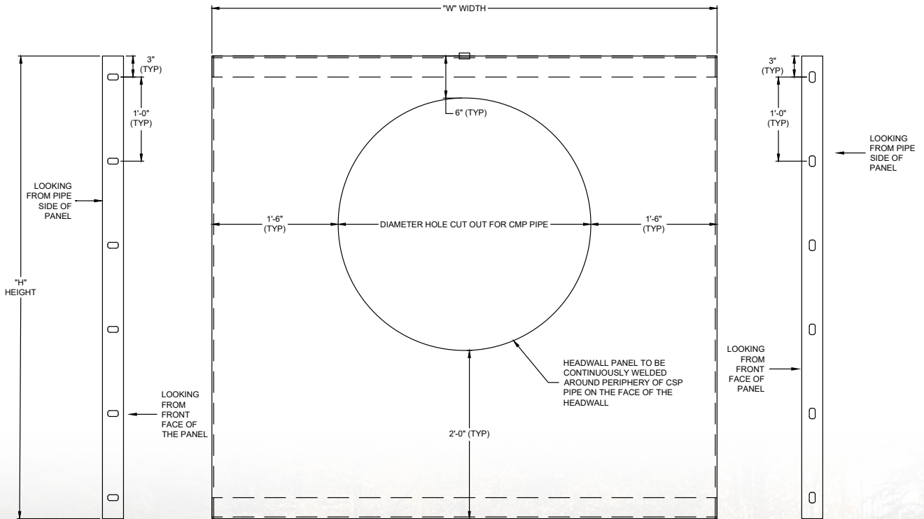
ELEVATION VIEW LOOKING FROM THE FRONT FACE OF THE PANEL
