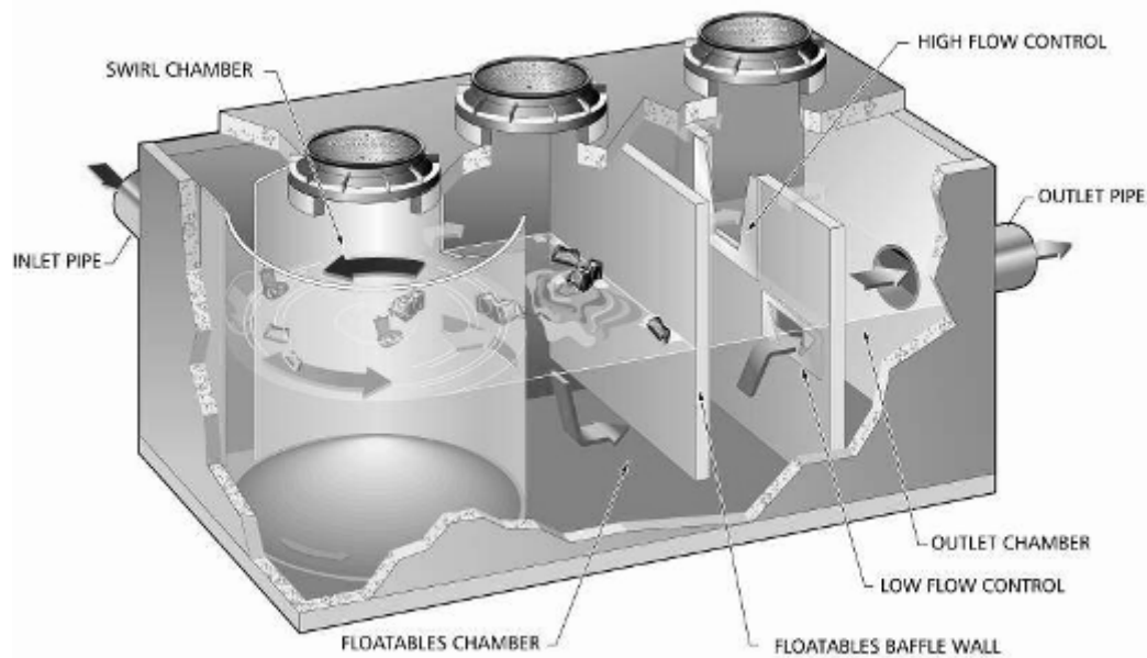
Figure 1 Standard Vortechs Stormwater Treatment System
