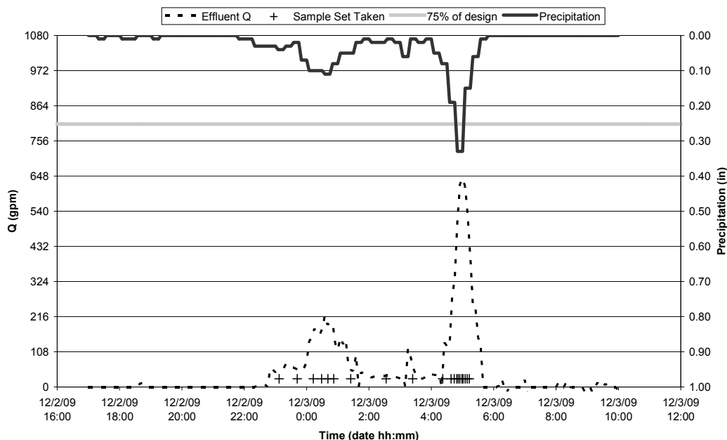
Event Hydrograph
