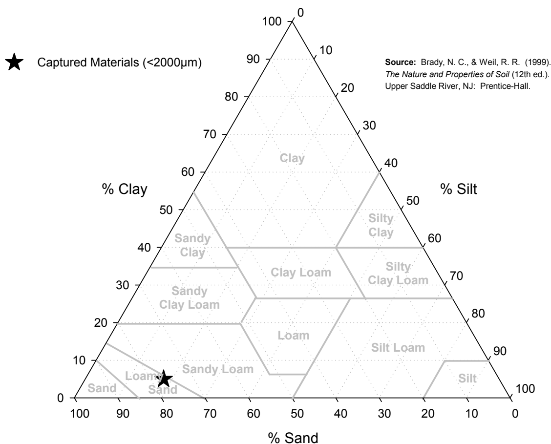
Figure 7 Textural triangle showing particle size analysis of materials captured in the Vortechs system
