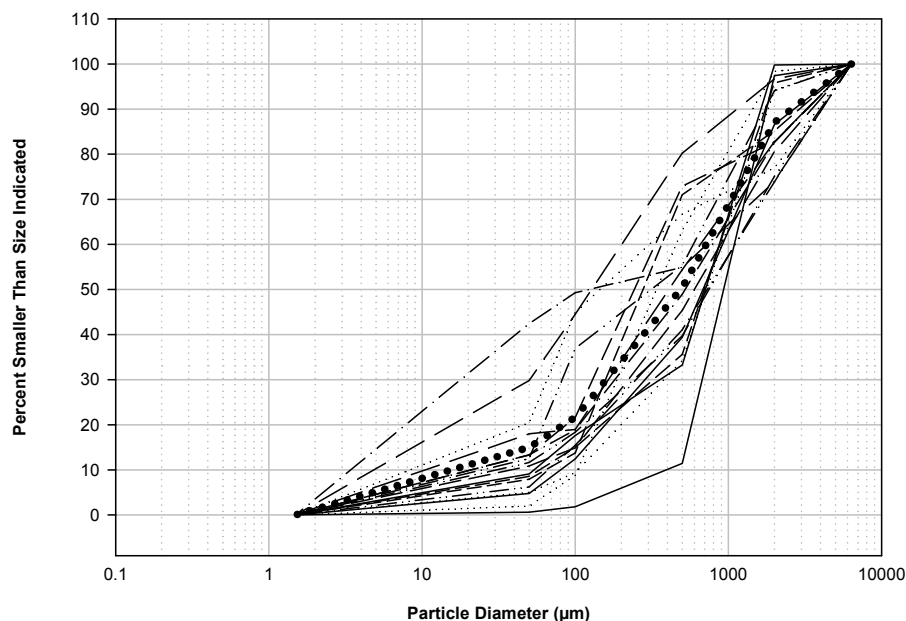
Figure 8 Influent particle size distribution generated using serial filtration covering 6350\mu\text{m} to 1.5\mu\text{m} particle size range; dashed line represents mean particle size distribution
