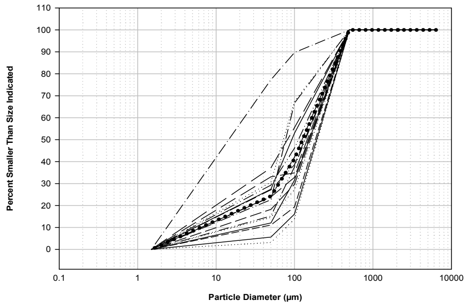
Figure 9 Influent particle size distribution generated using serial filtration covering 500μm to 1.5μm particle size range; dashed line represents mean particle size distribution
