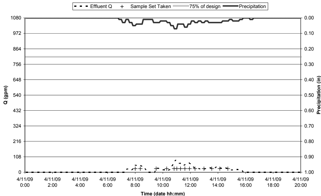
Event Hydrograph
