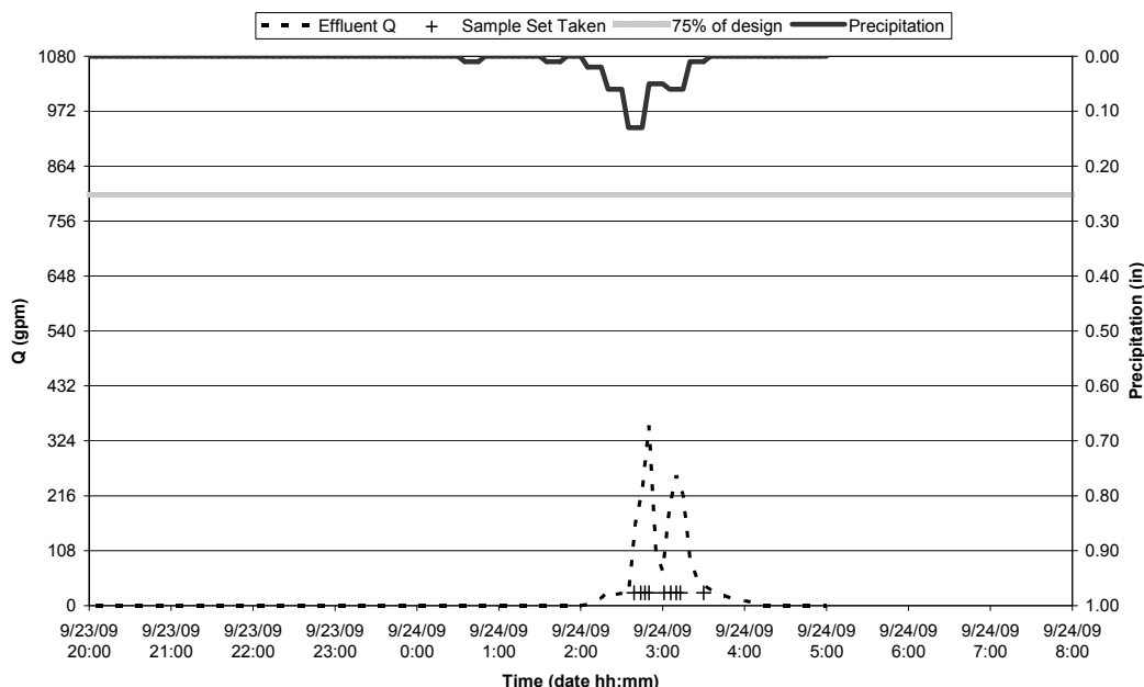
Event Hydrograph
