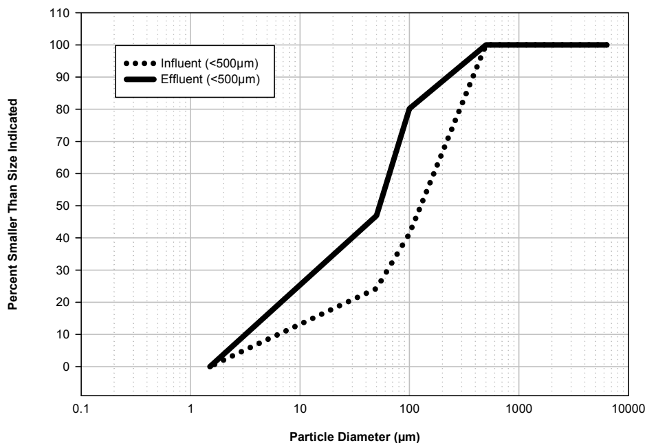
Figure 11 Comparison of mean influent and effluent particle size distributions generated using serial filtration covering 500 \mu\text{m} to 1.5 \mu\text{m} particle size range
