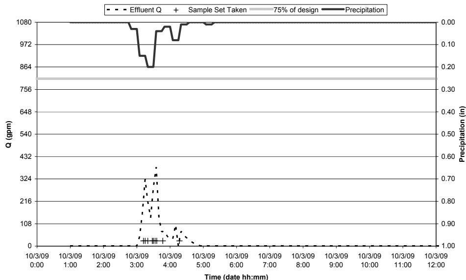
Event Hydrograph
