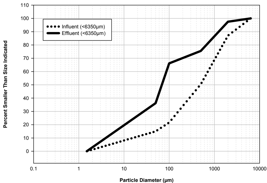
Figure 10 Comparison of mean influent and effluent particle size distributions generated using serial filtration covering 6350μm to 1.5μm particle size range
