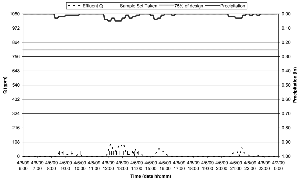
Event Hydrograph
