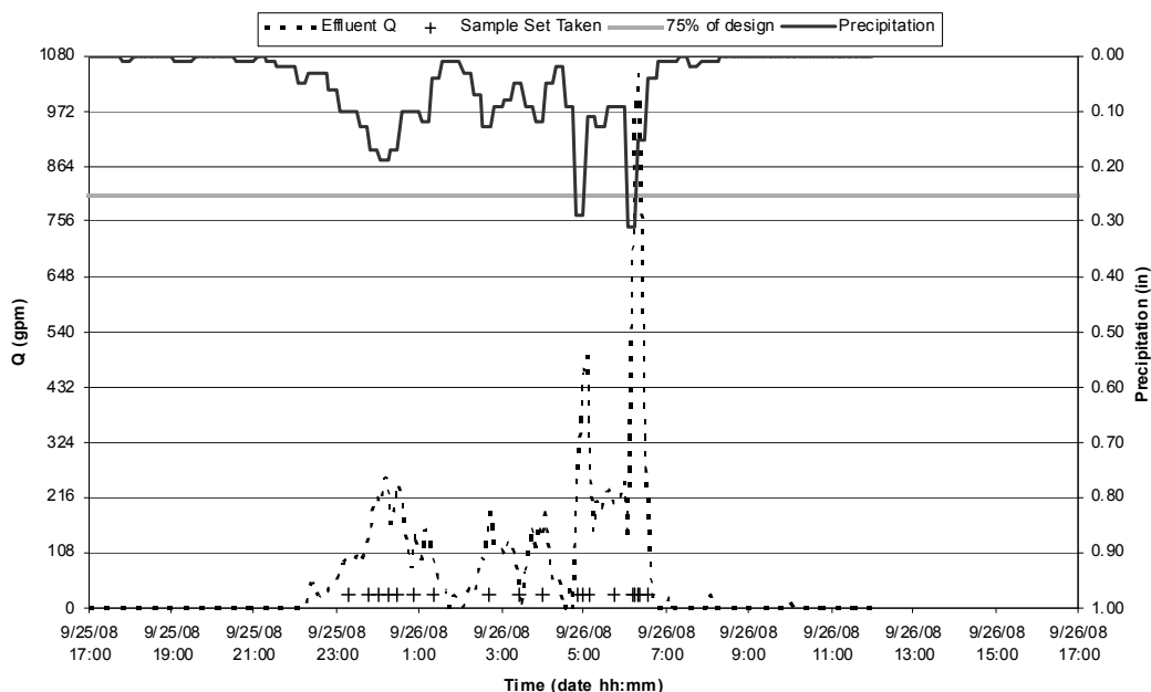
Event Hydrograph
