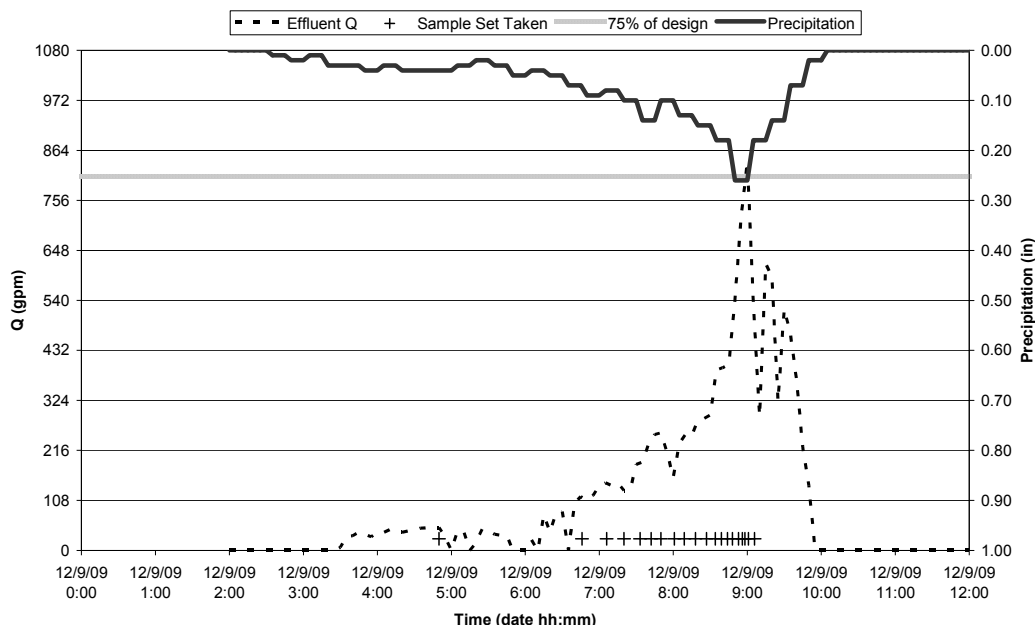
Event Hydrograph
