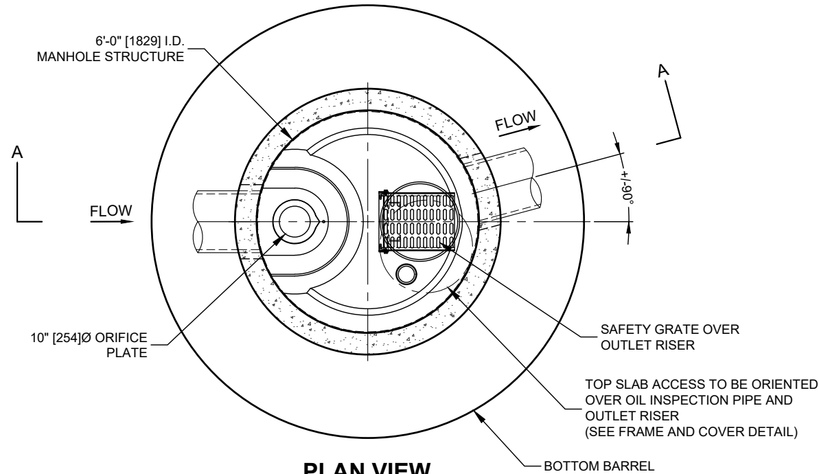
PLAN VIEW TOP SLAB NOT SHOWN
