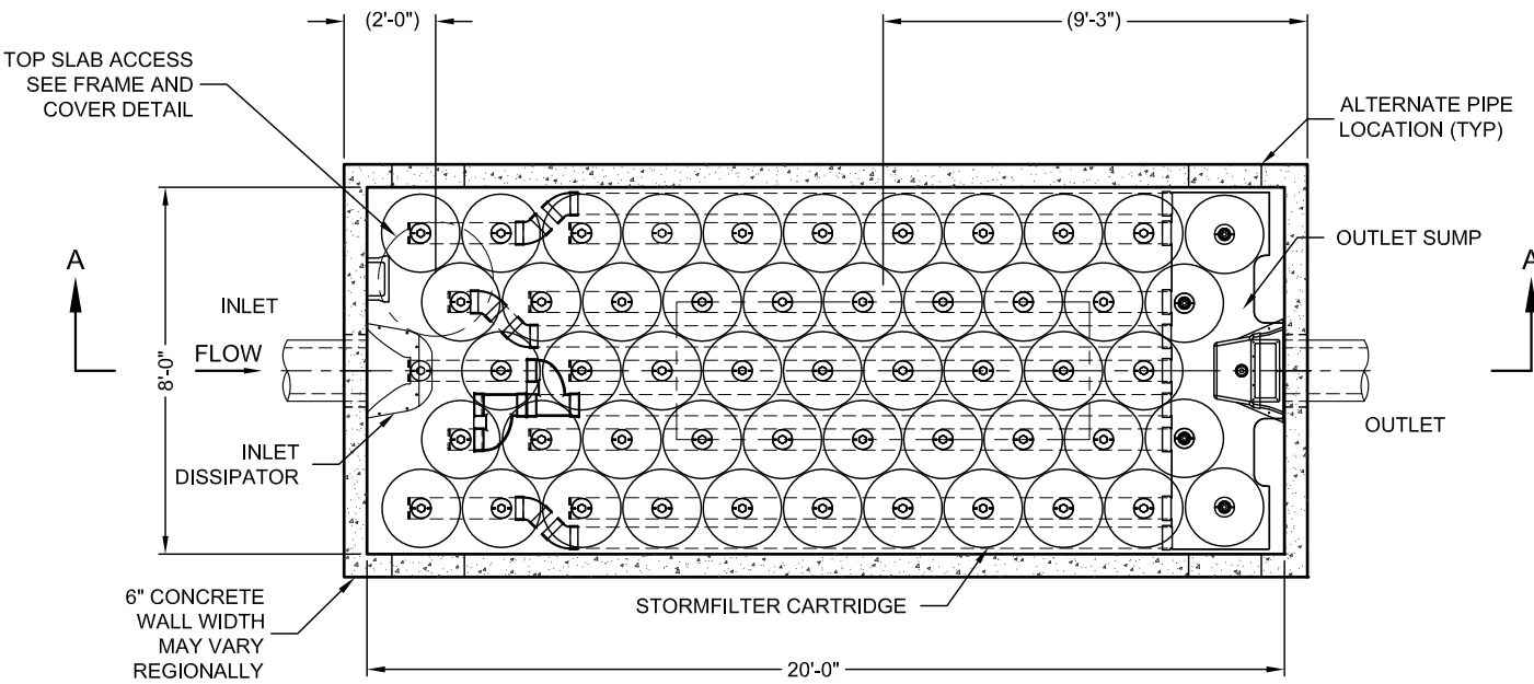
PLAN VIEW VAULT STYLE: OUTLET SUMP (NIB)
