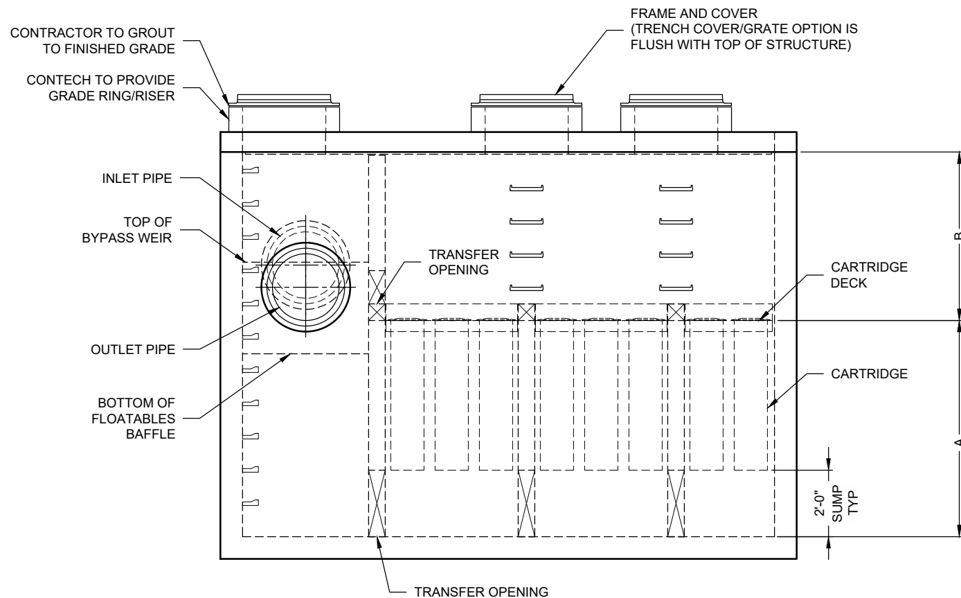
ELEVATION VIEW
