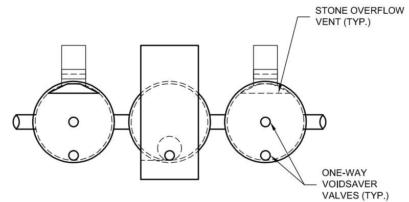
RIGHT VIEW
