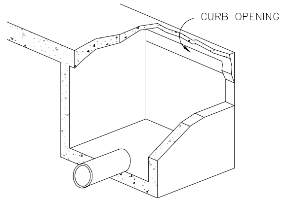
ISO VIEW
