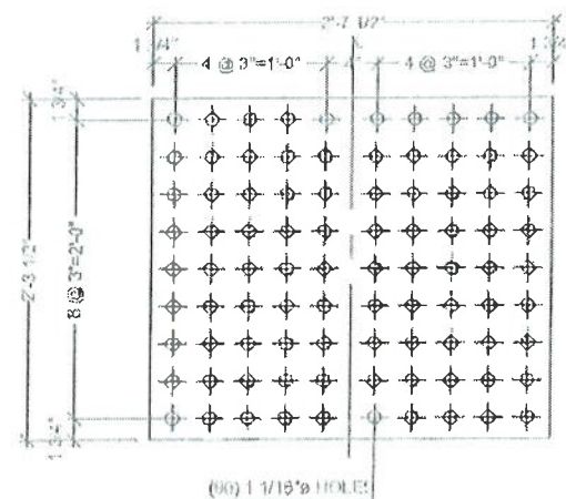
WEB SPLICE PLATE
