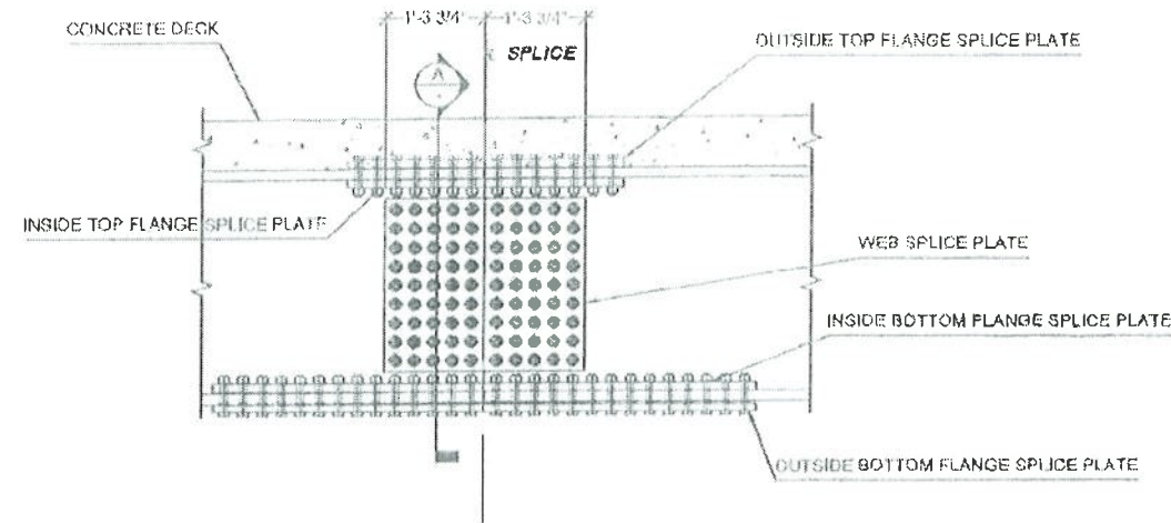
STRINGER SPLICE DETAILS
