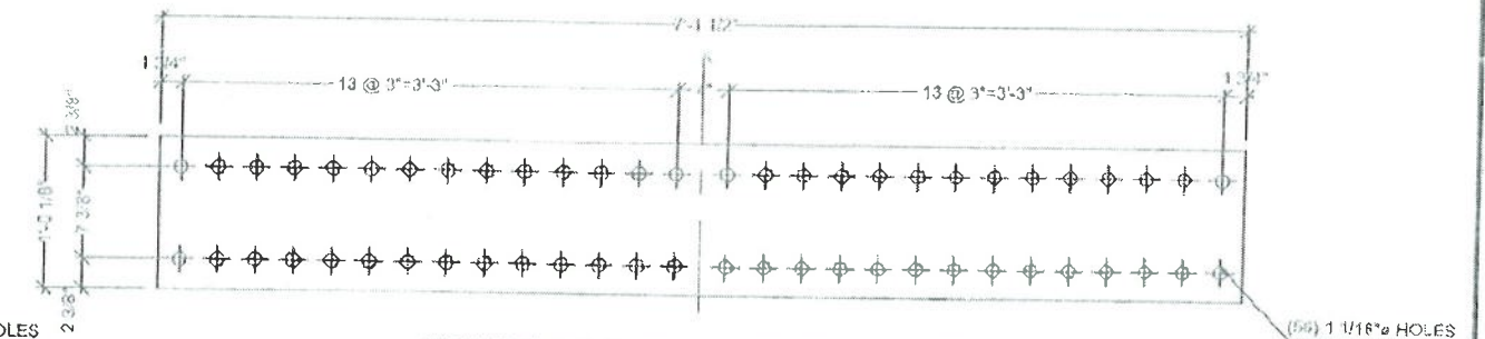
OUTSIDE BOTTOM FLANGE SPLICE PLATE
