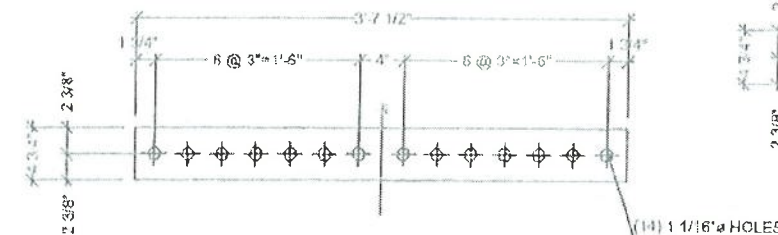
INSIDE TOP FLANGE SPLICE PLATE
