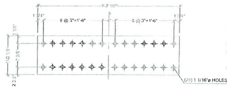
OUTSIDE TOP FLANGE SPLICE PLATE
