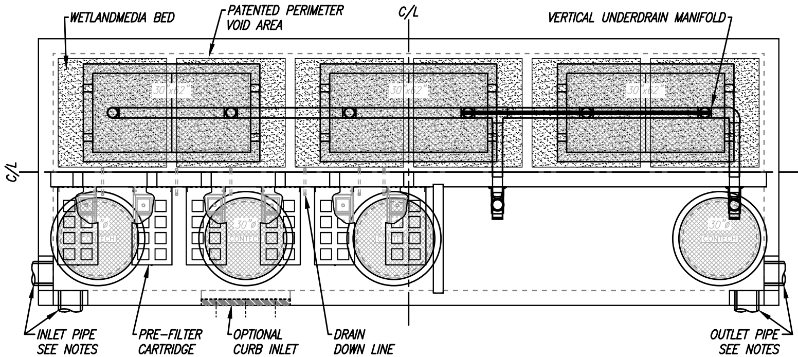
PLAN VIEW
