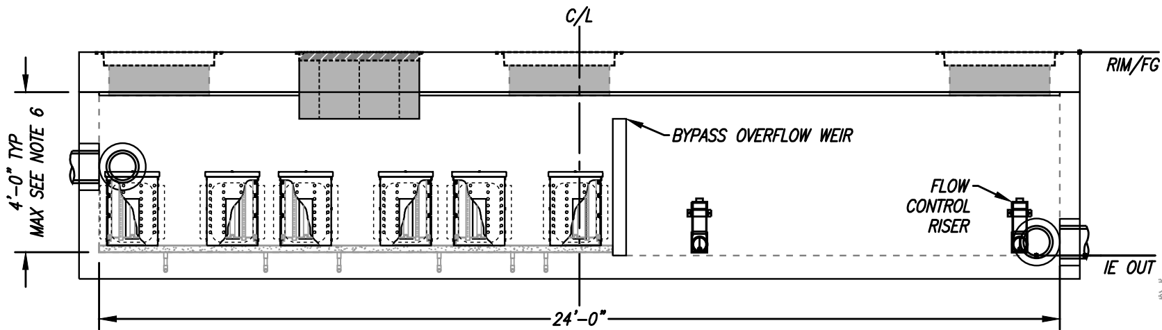
ELEVATION VIEW
