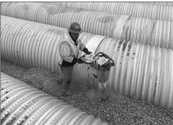
Examples of compaction with vibratory equipment around the culvert pipe.
