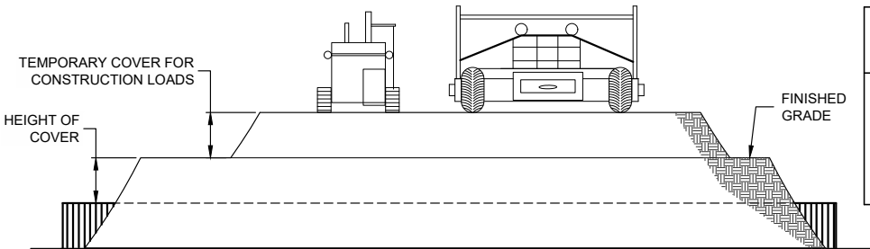
Examples of heavy construction equipment that may require additional minimal cover. Contech can help evaluate minimum cover for the installation contractor for all the equipment on the site.
