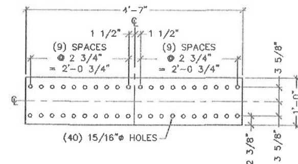
(4) OUTSIDE BTM FLANGE SPICE PLATE REQ'D
