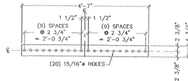
(8) INSIDE BTM FLANGE SPICE PLATE REQ'D
