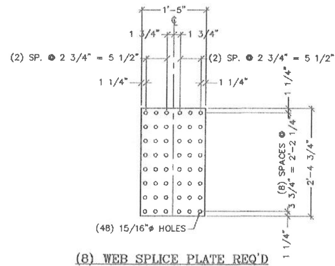
STRINGER SPICE DETAILS
