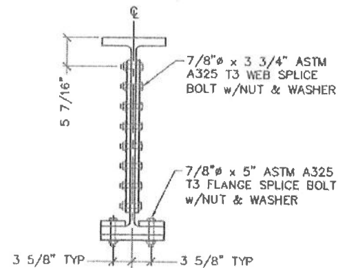
SECTION A
