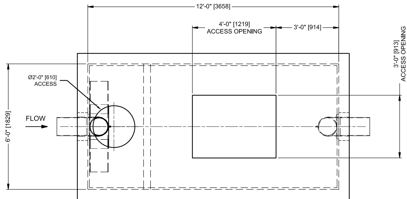
PLAN VIEW (MEDIA NOT SHOWN FOR CLARITY)
