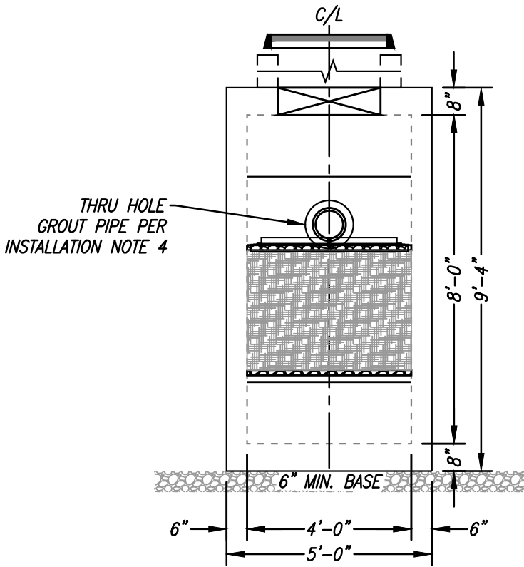
END VIEW
