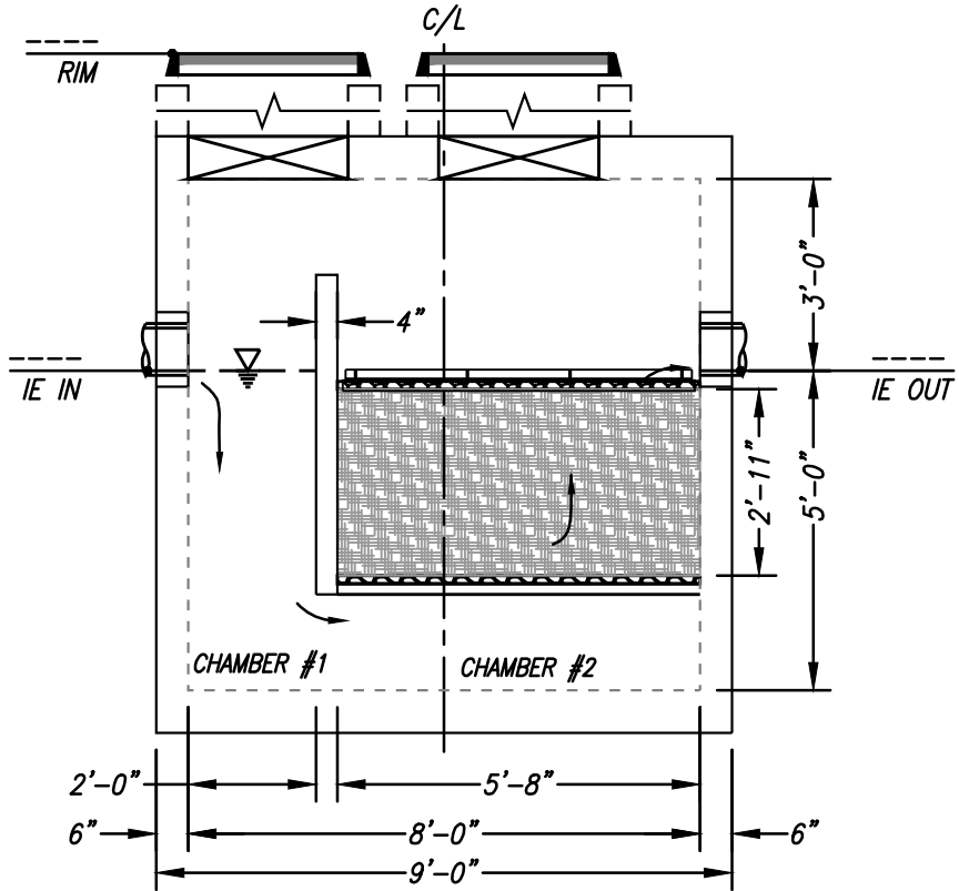
ELEVATION VIEW
