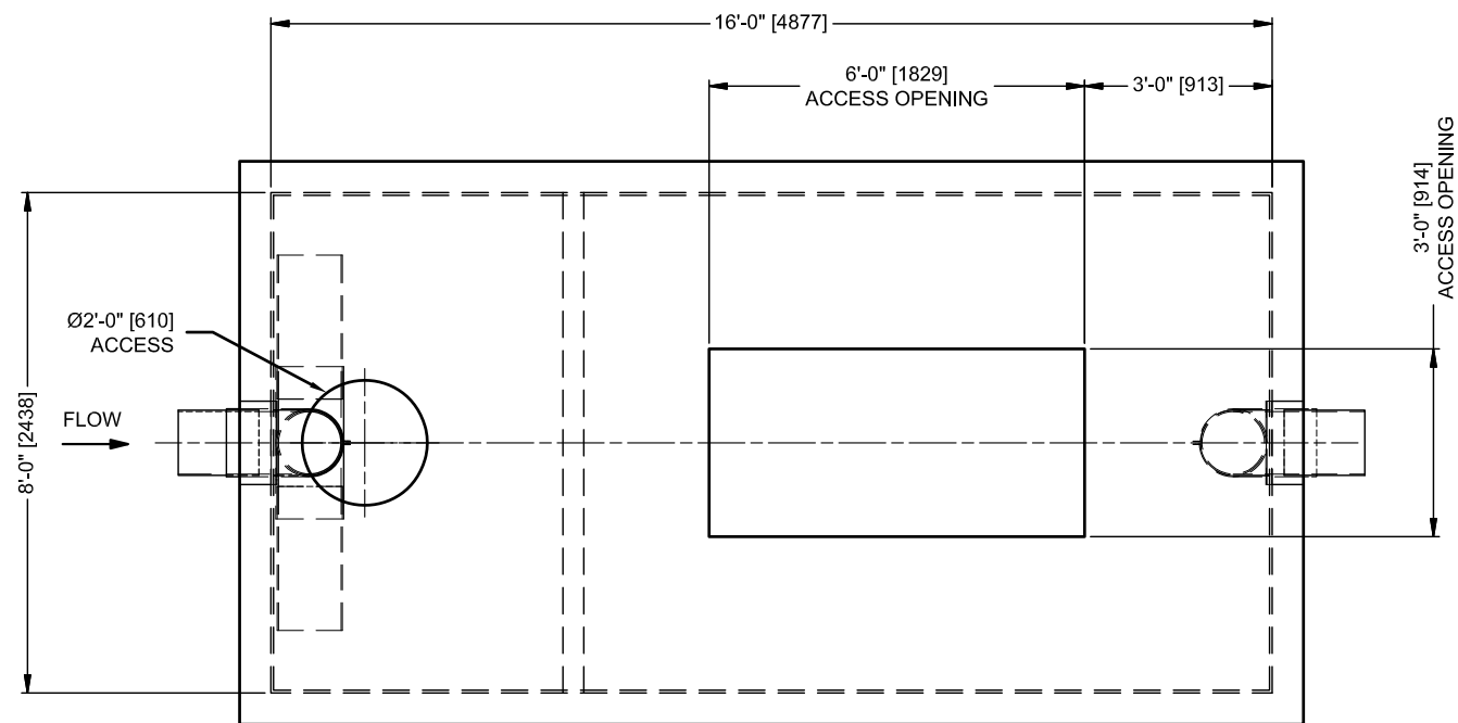
PLAN VIEW (MEDIA NOT SHOWN FOR CLARITY)
