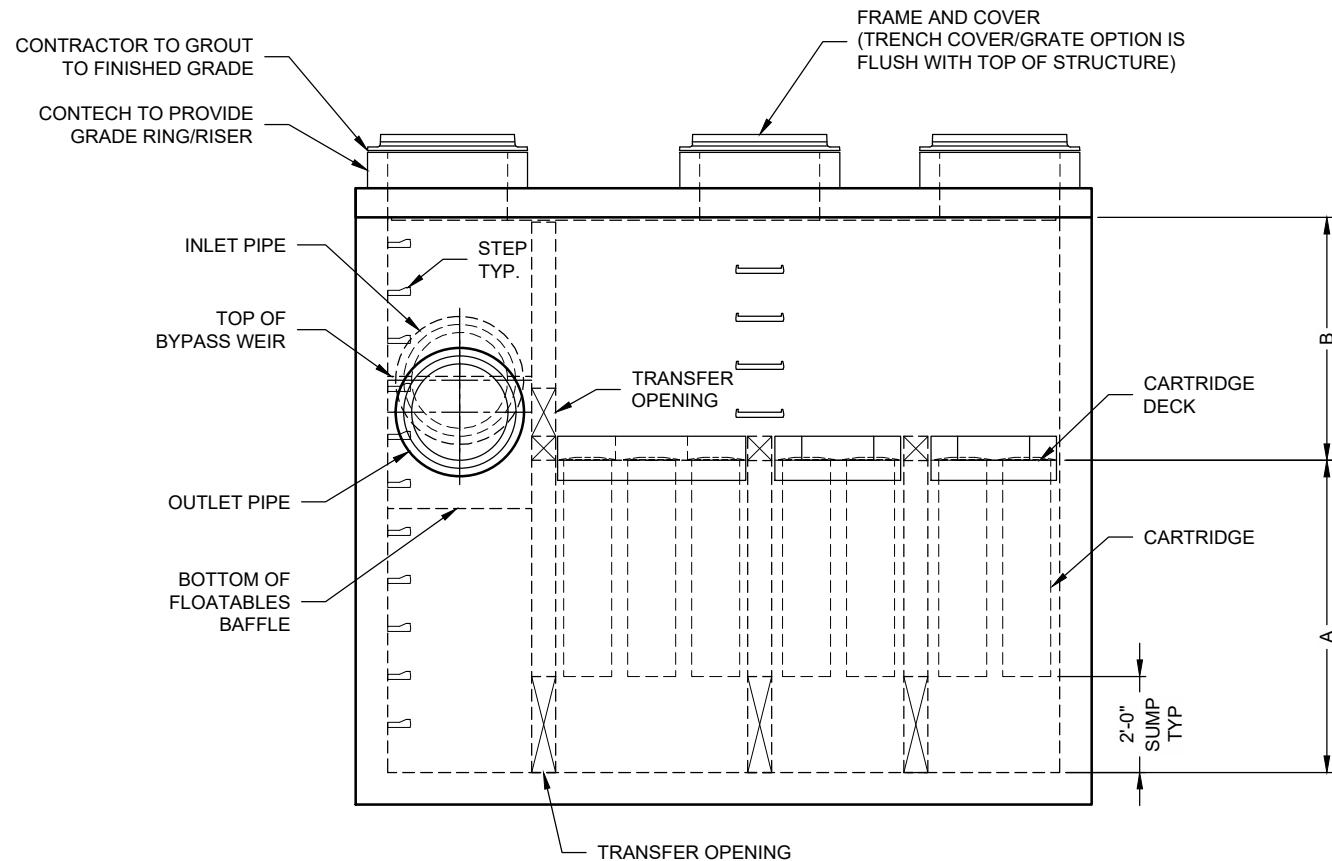
ELEVATION VIEW
