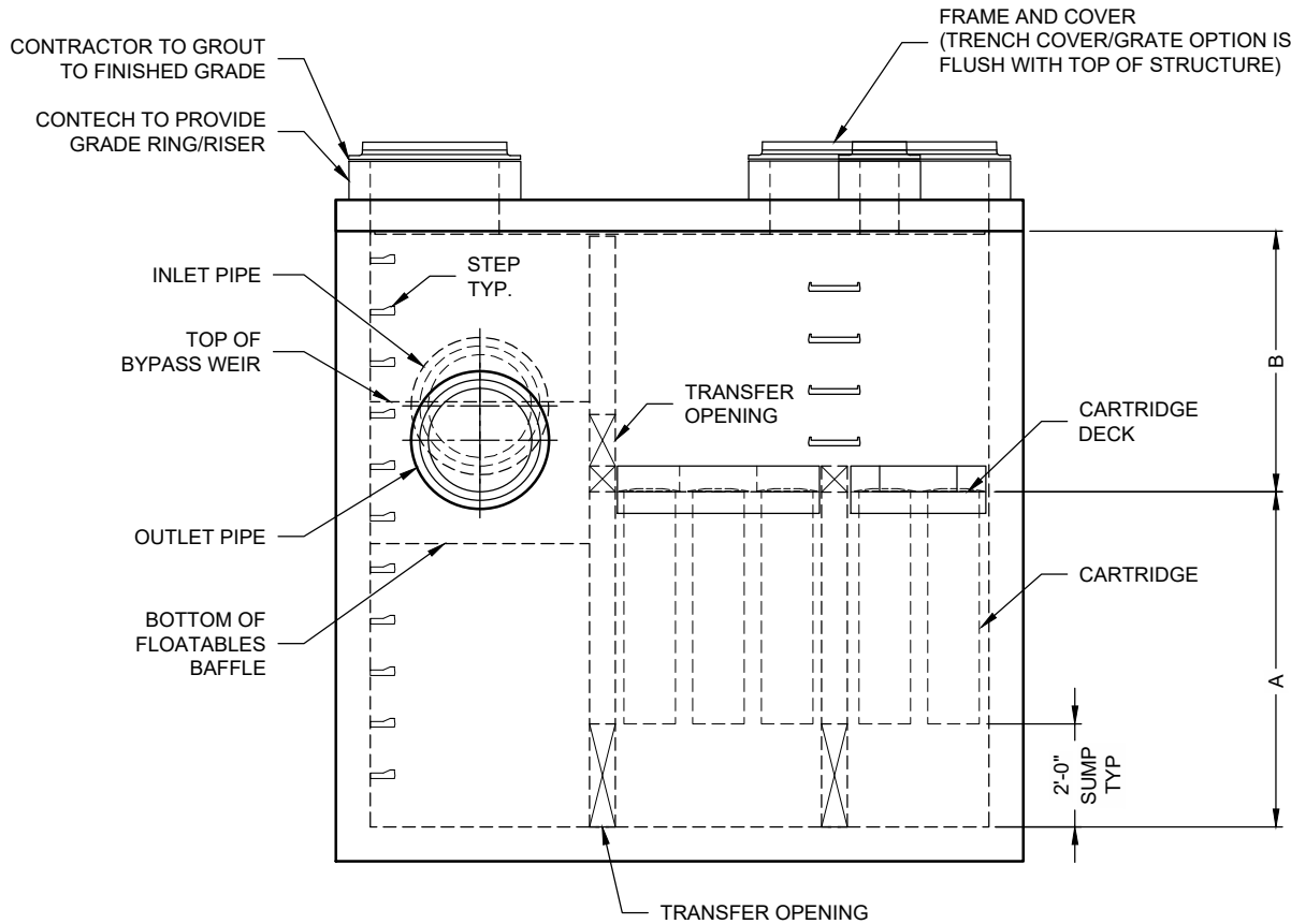
ELEVATION VIEW
