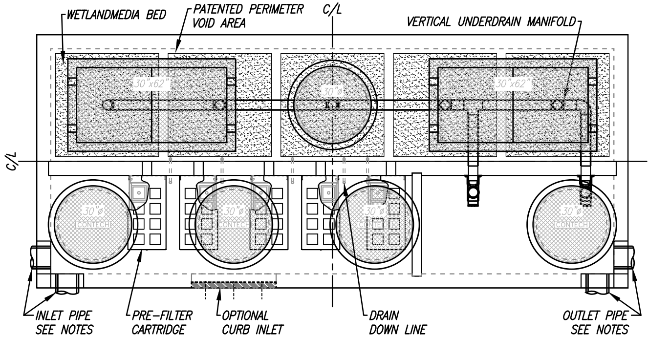
PLAN VIEW
