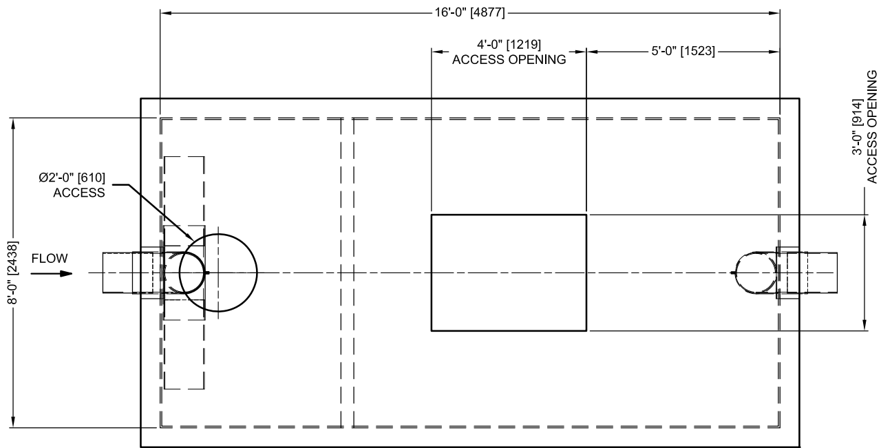
PLAN VIEW (MEDIA NOT SHOWN FOR CLARITY)
