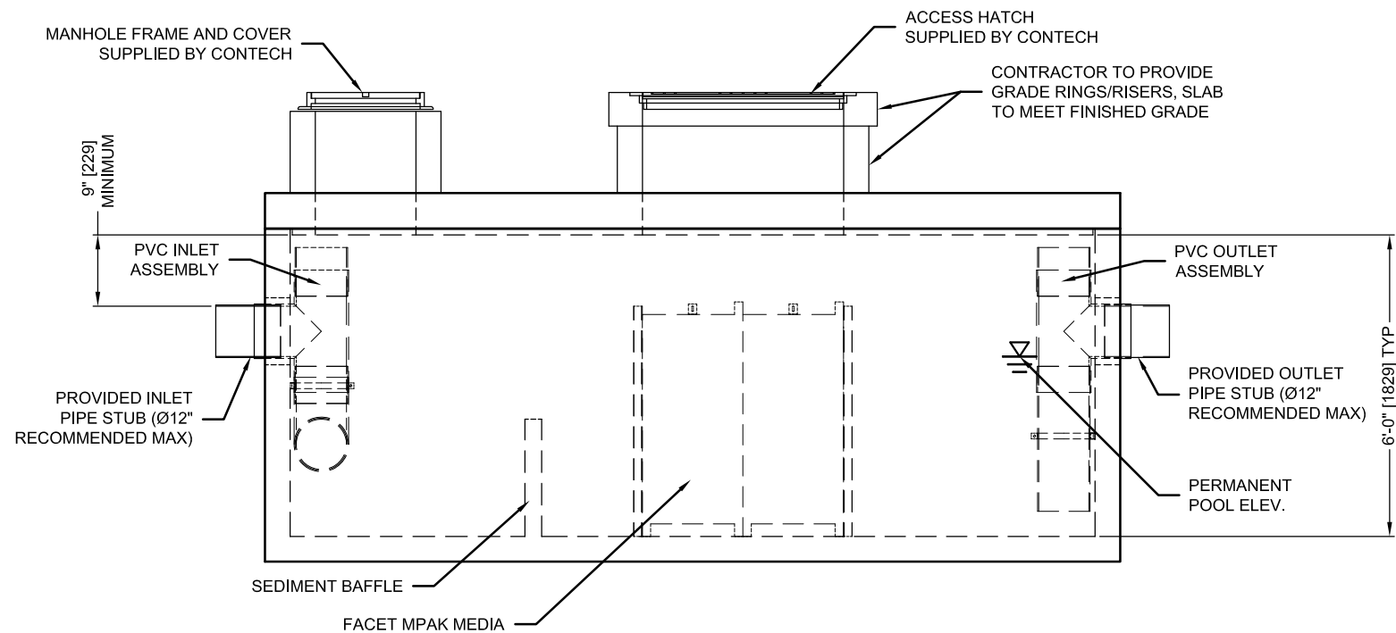
ELEVATION VIEW
