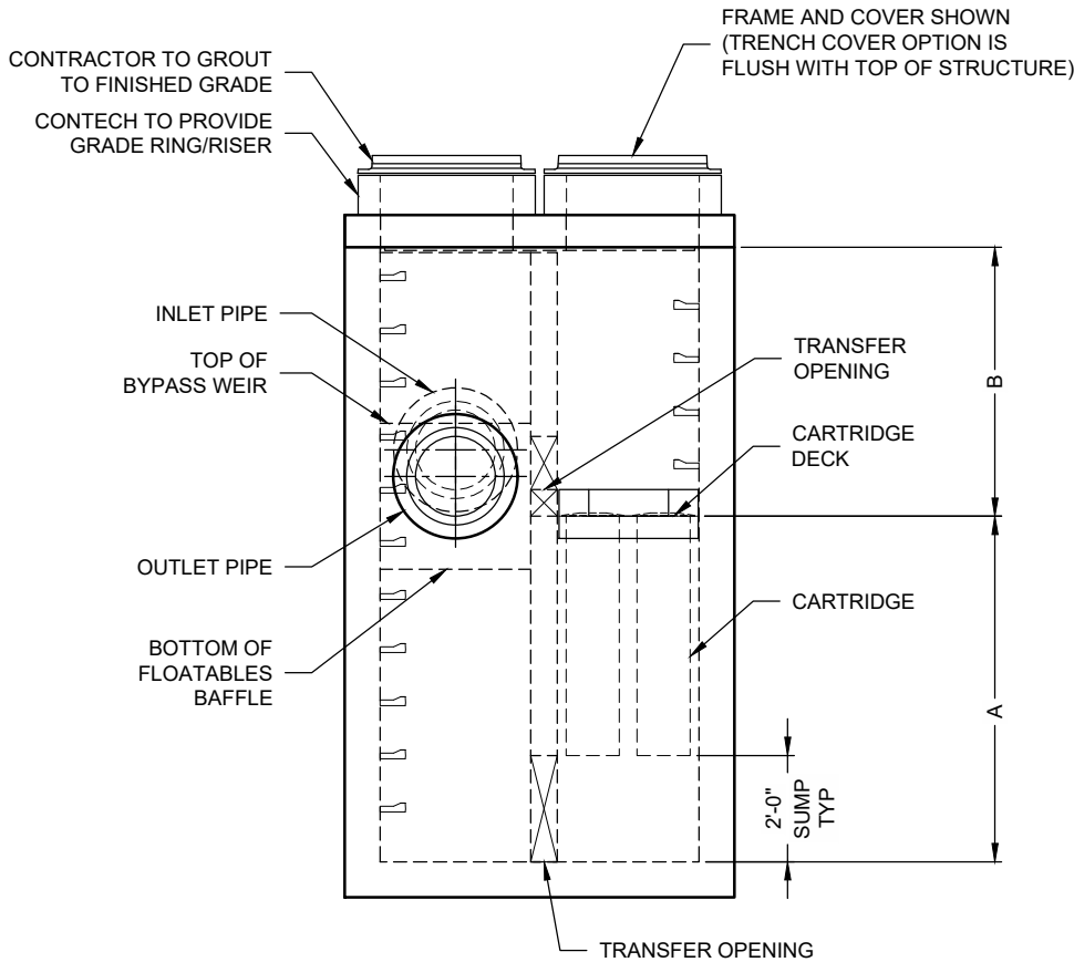
ELEVATION VIEW
