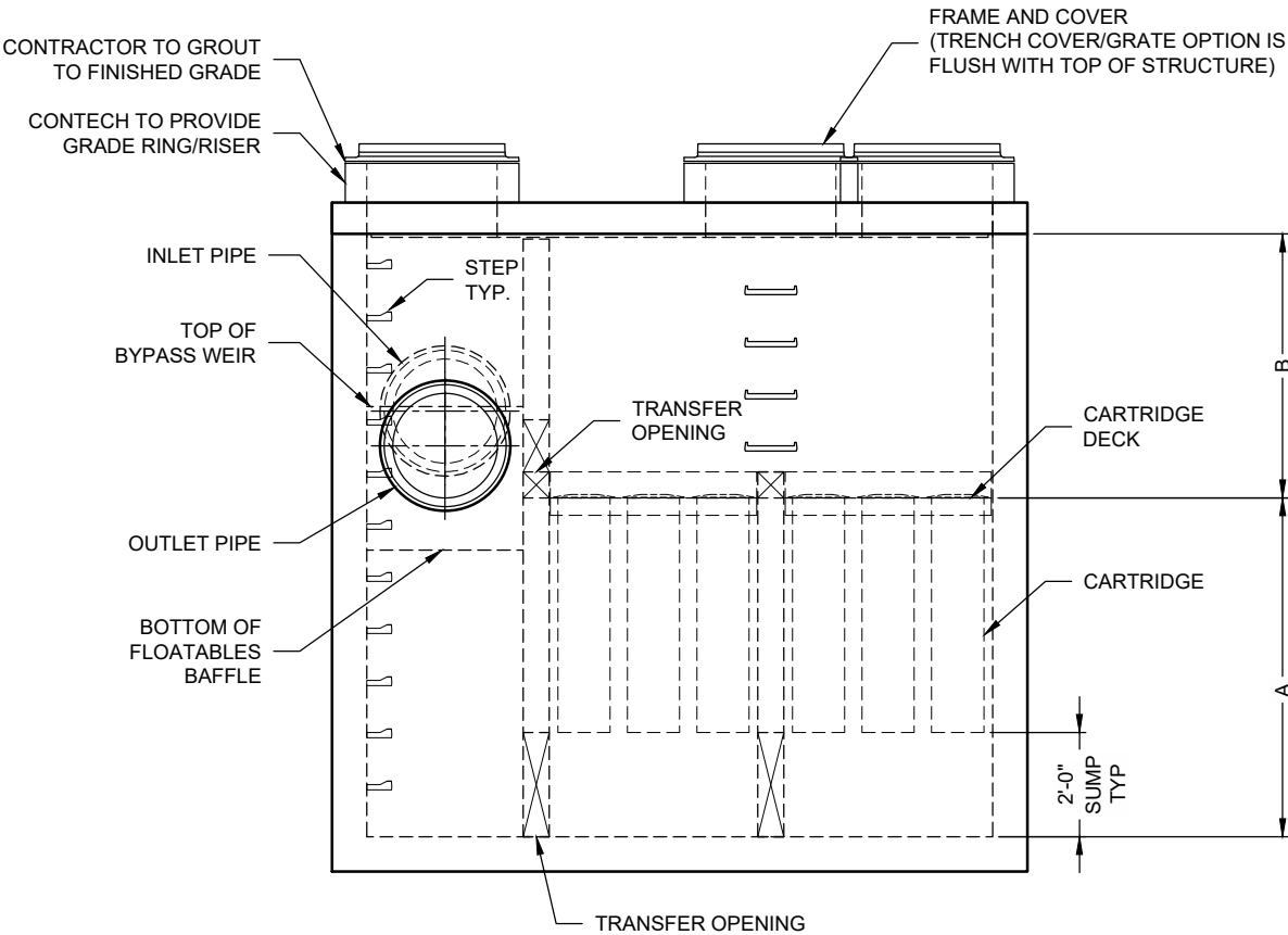
ELEVATION VIEW
