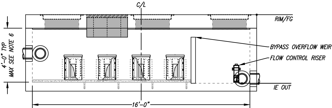
ELEVATION VIEW
