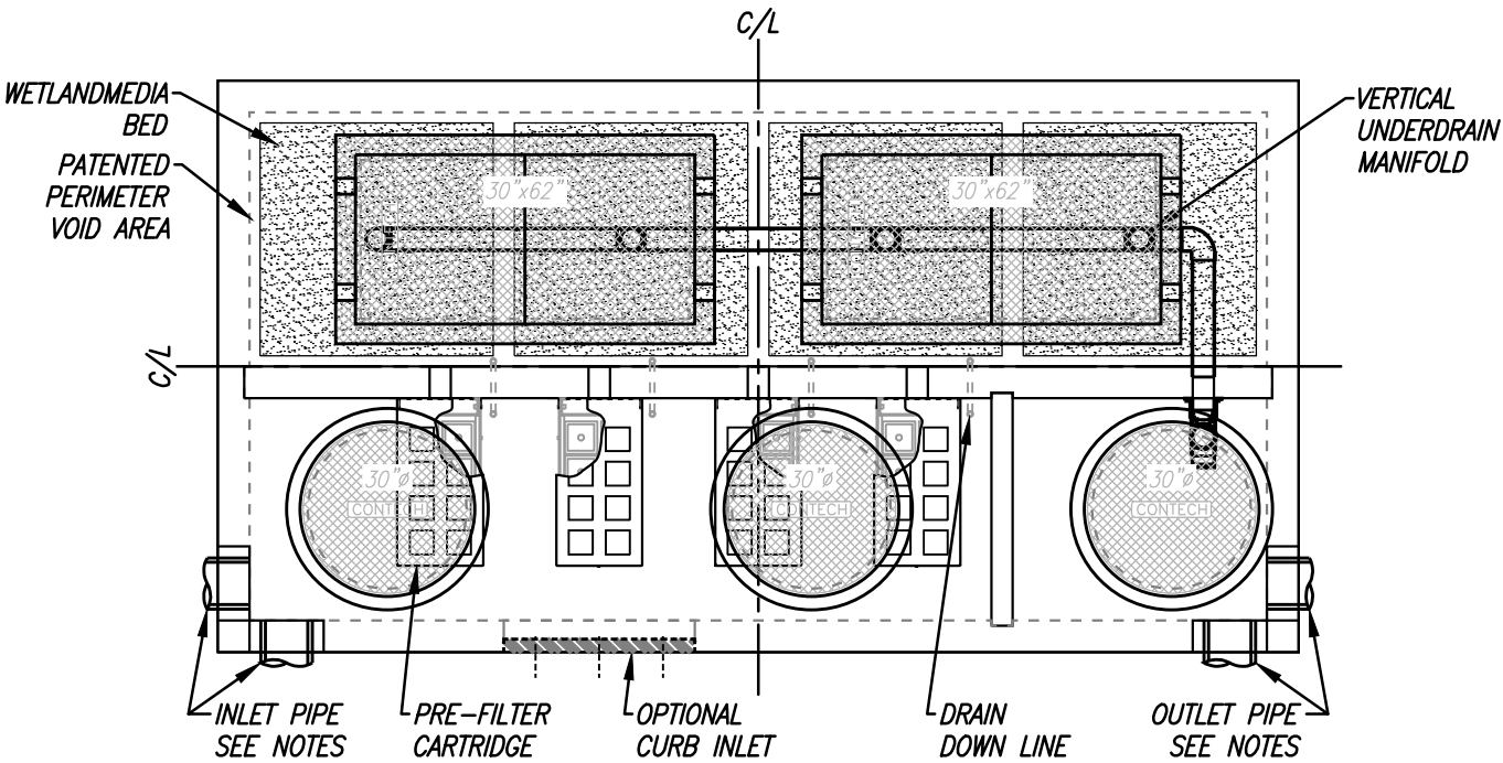
PLAN VIEW
