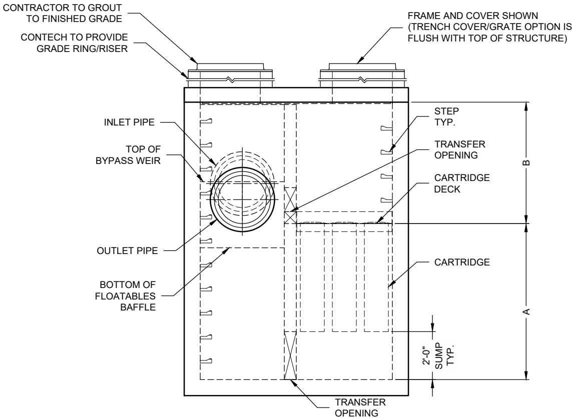
ELEVATION VIEW
