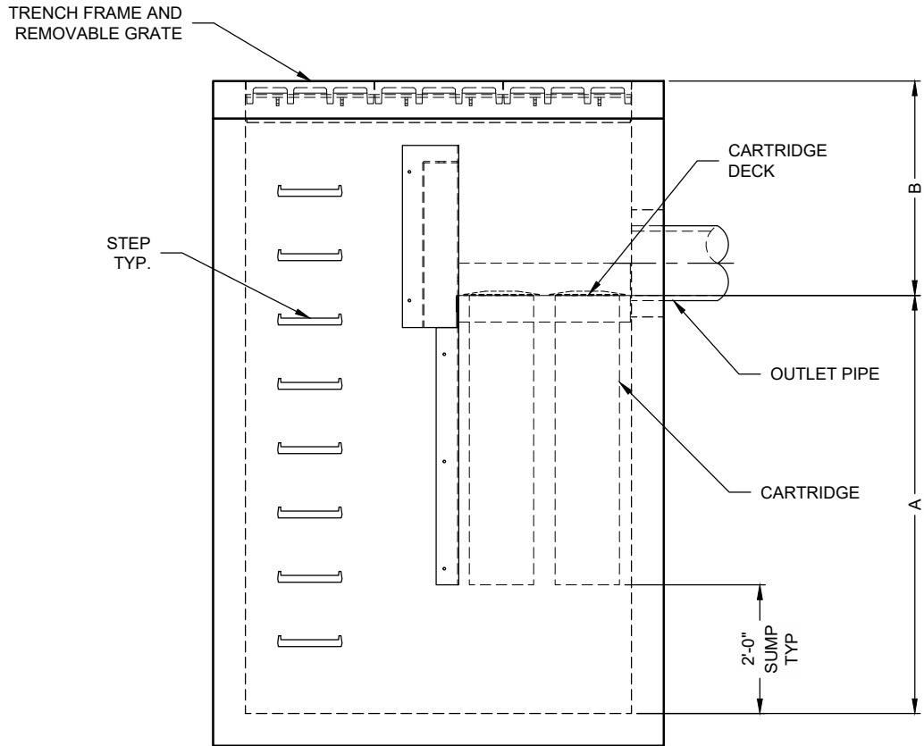
ELEVATION VIEW
