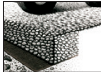
Geotex® "ST" series of woven geotextiles can reduce aggregate thickness in unpaved roads by as much as 50%.
