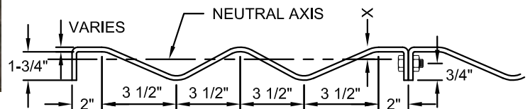
Section B-B
