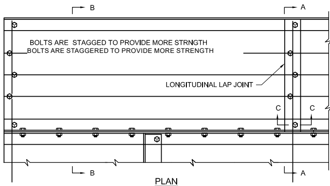
2-Flange Lap Joint
