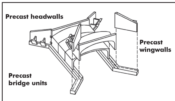
Complete Precast System
